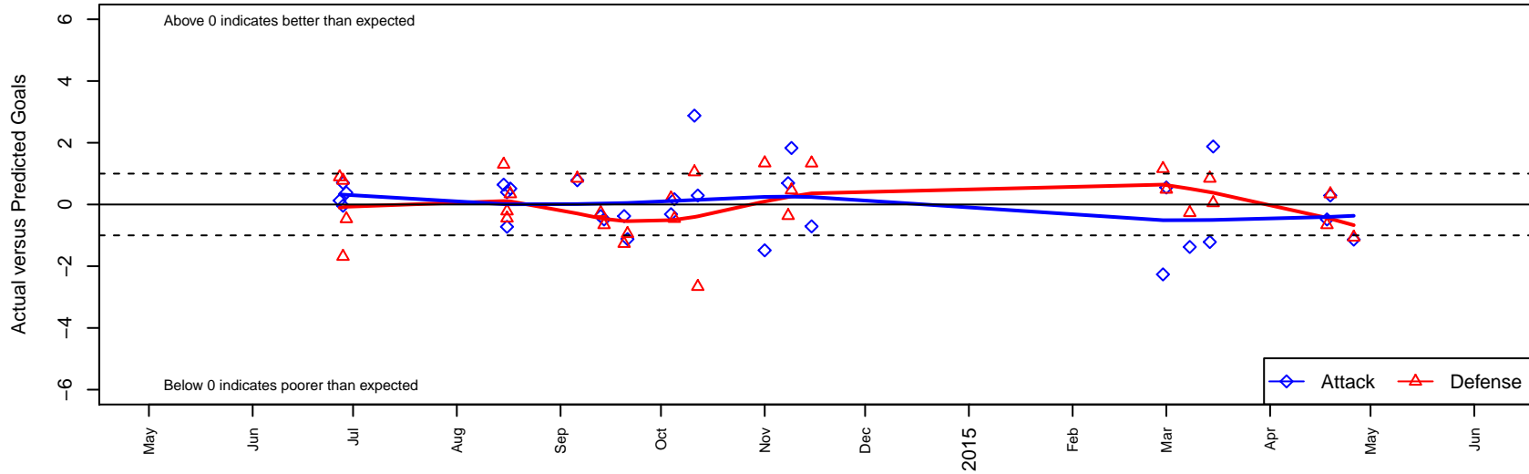
Washington Timbers Green G00 Dots are actual minus expected GF (blue circles) and GA (red triangles). Blue line is smoothed change in attack strength. Red is smoothed change in defense strength.
